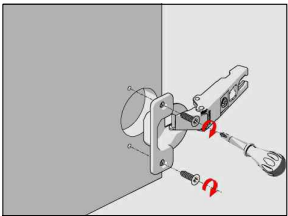
Hinge adjustment
